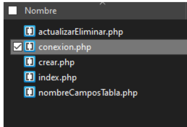
Figure 1. Software files
